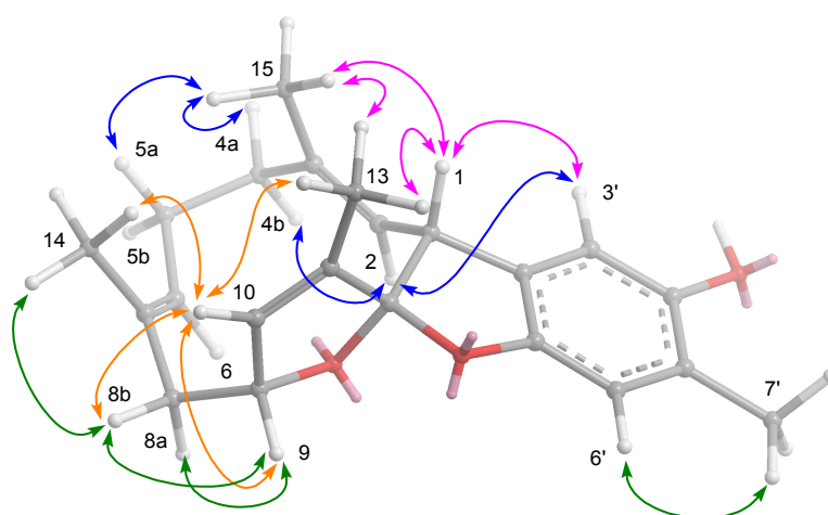
Figure 4. Selected NOESY correlations of 1 .
