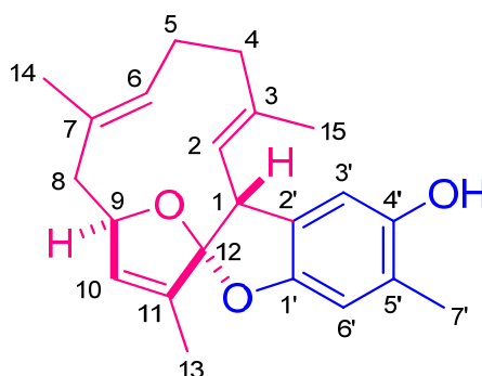
Figure 2. The structure of capilloquinol ( 1 ).
