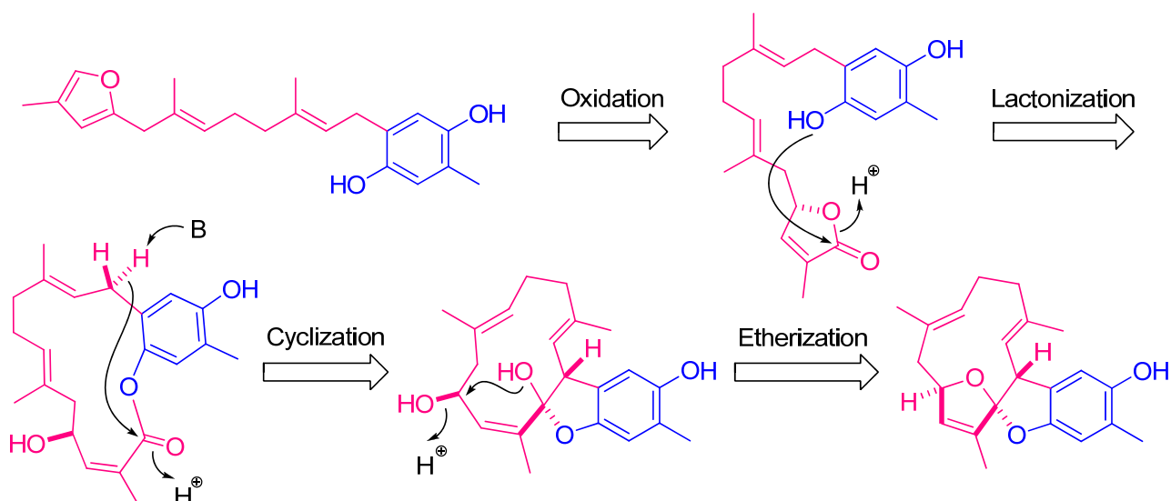
Scheme 1. Possible biogenetic pathway for 1 .
