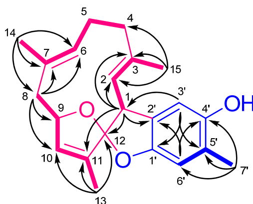
Figure 3. Key ^1\text{H} - ^1\text{H} COSY (—) and HMBC (→) correlations of 1 .
